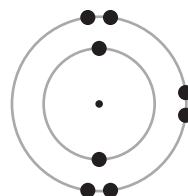
oxygen atom
